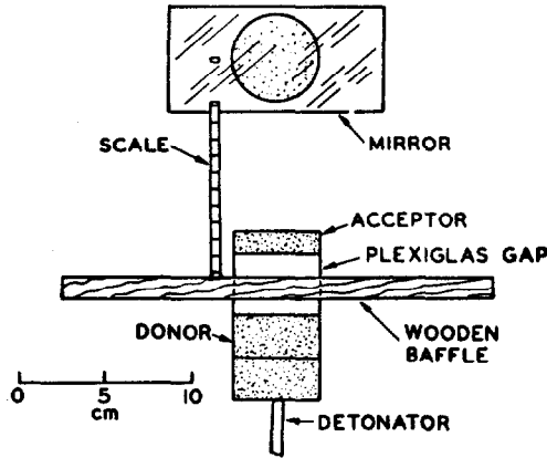
Fig 26 The modified gap test
